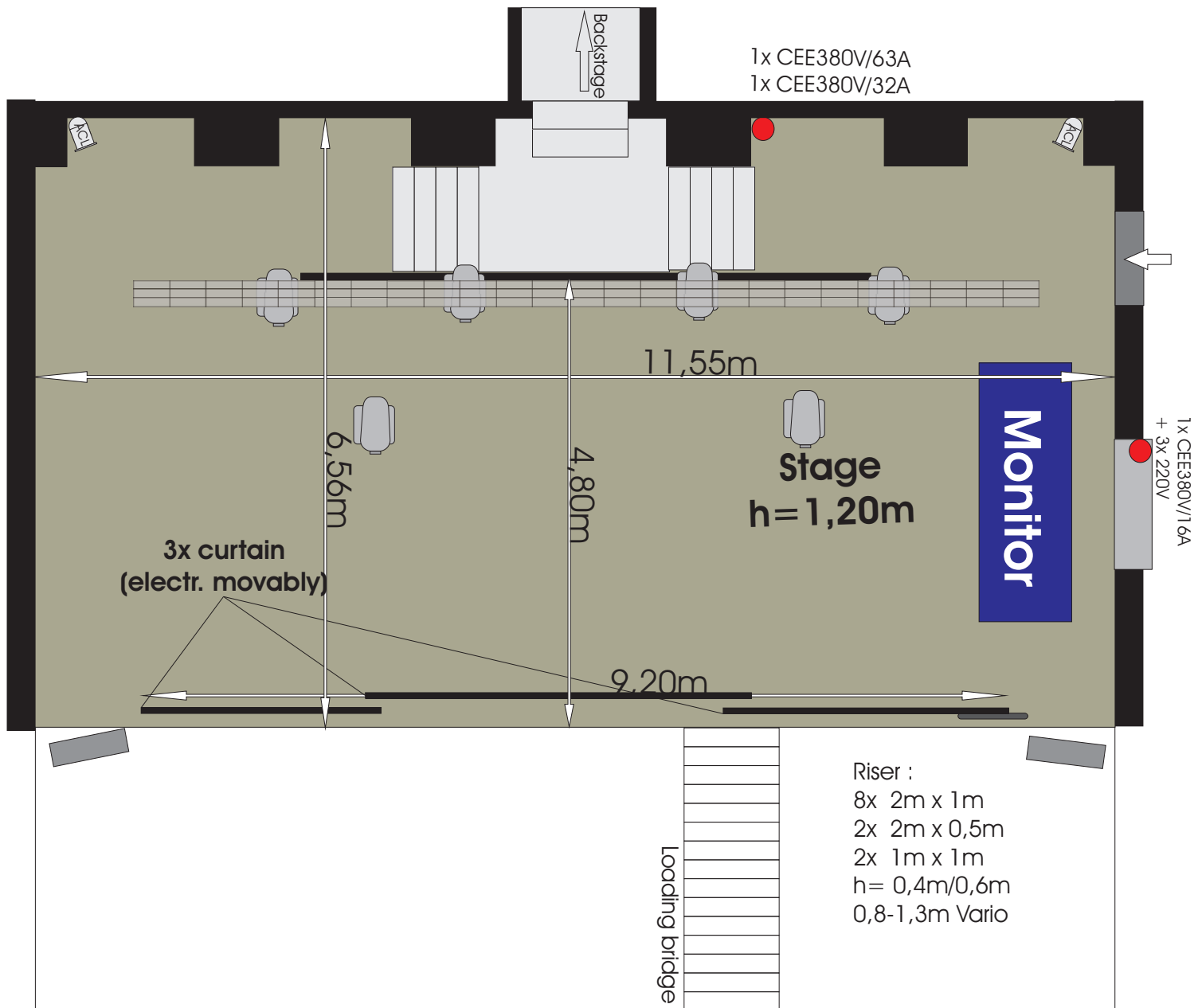
Plan view "Stage" (without crane/Lightkonstruktion)
