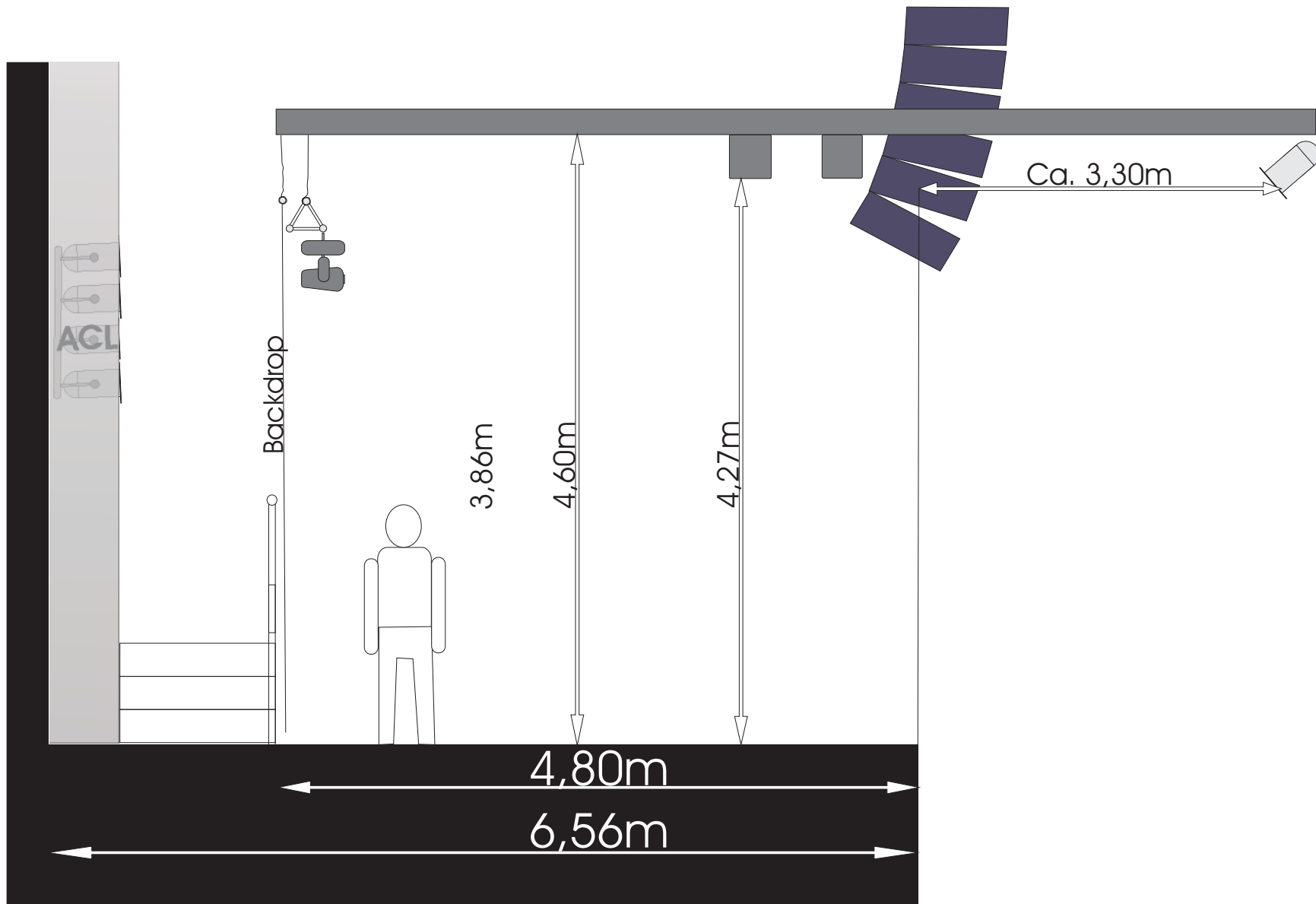
Side view
