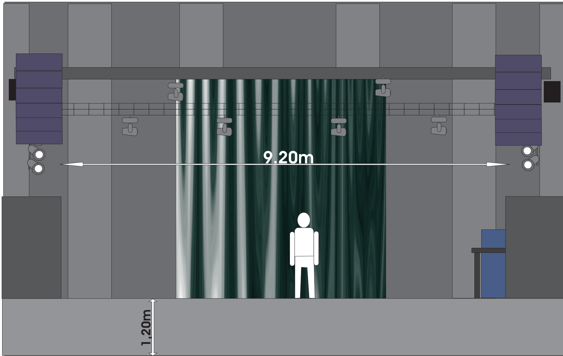
Frontal view
